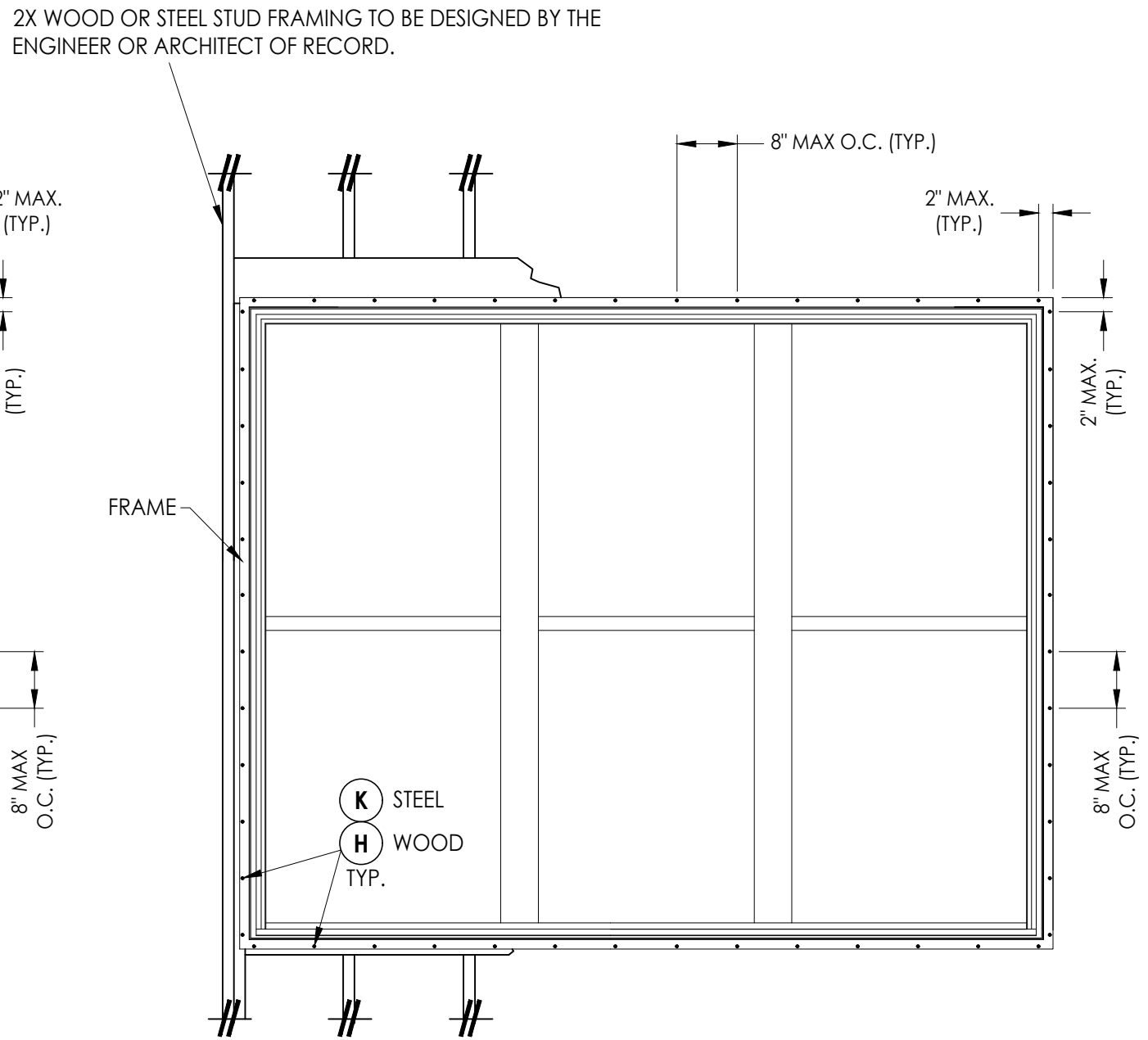
FRAME ANCHORING
