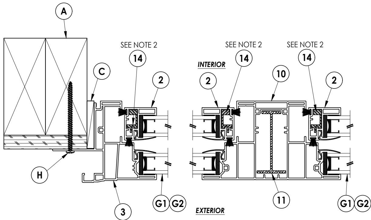
1 HORIZONTAL CROSS SECTION Stud Construction
